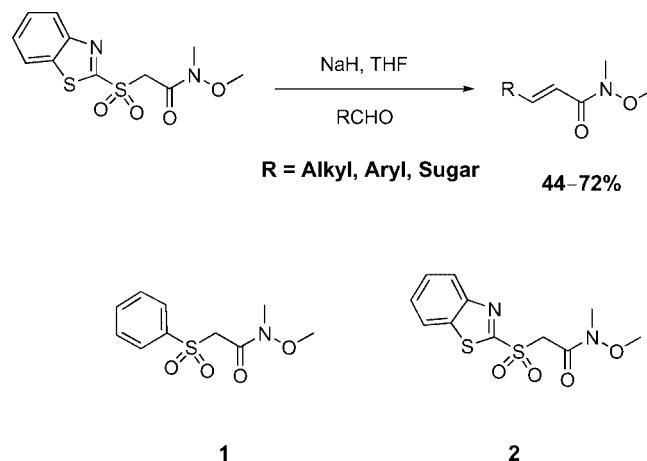
Figure 1. Reaction of reagent 2 with various aldehydes to give \alpha,\beta -unsaturated Weinreb amides.
