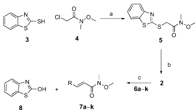
Scheme 1. Reagents and conditions: a: \text{Na}_2\text{CO}_3 , \text{H}_2\text{O} 14 h; b: \text{Na}_2\text{WO}_4 , \text{H}_2\text{O}_2 , MeOH, 16 h; c: NaH, THF then RCHO ( 6a–k ), room temp., 24 h.
